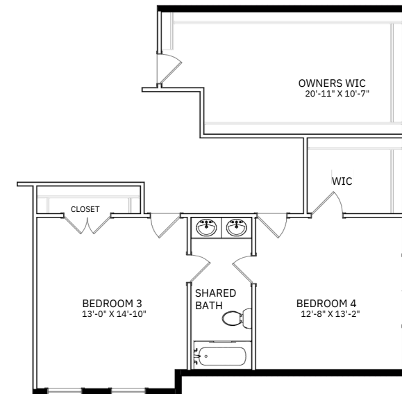
OPT. LAYOUT W/ JACK & JILL BATH
